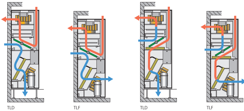
Free cooling and mixed mode
