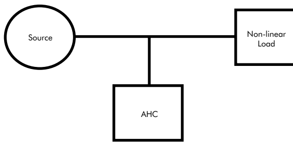
Figure 3 - Parallel conditioner
