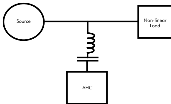
Figure 4 - Hybrid conditioner
