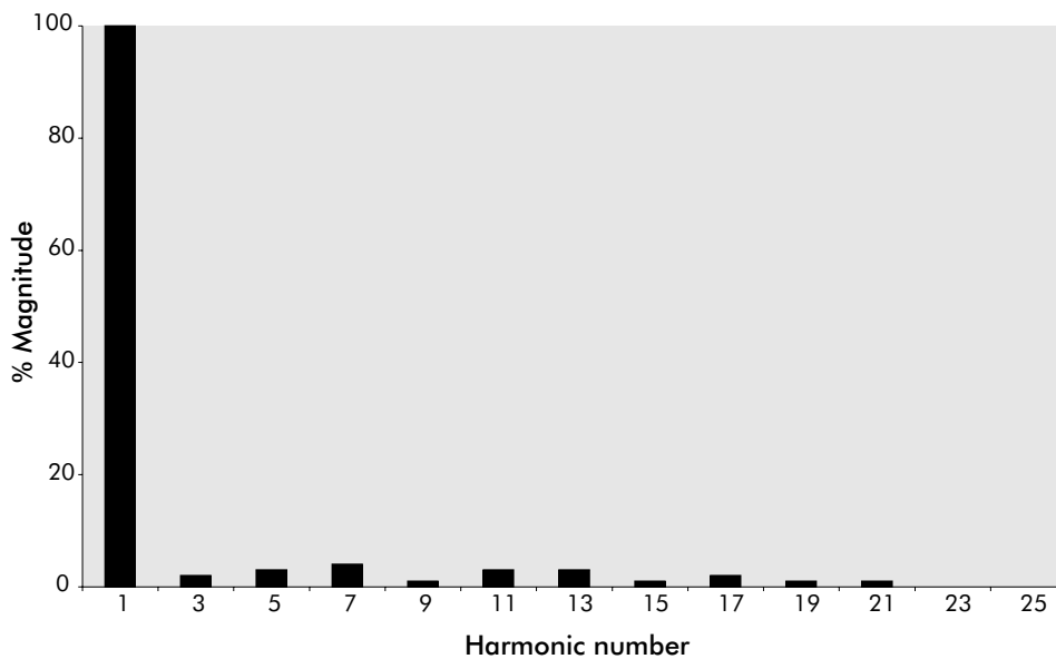
Figure 12 - Corrected variable speed drive type load
