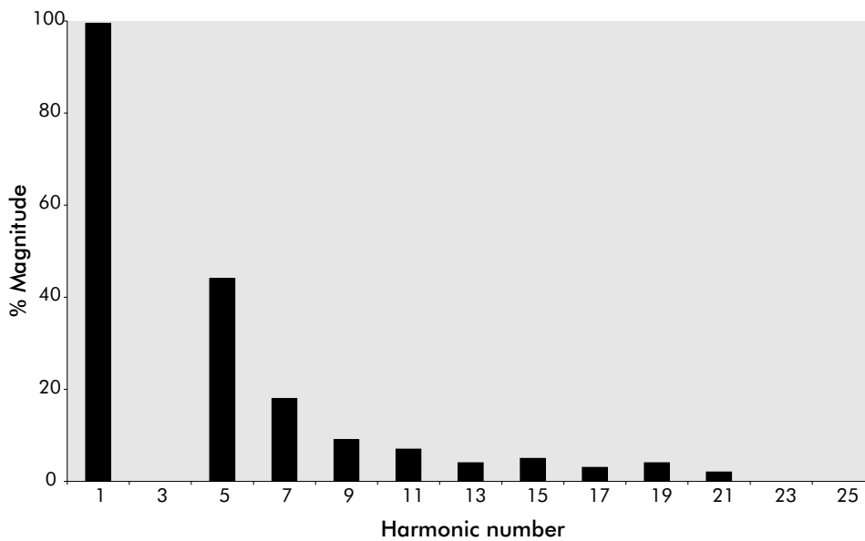
Figure 10 - Partially corrected PC type load
