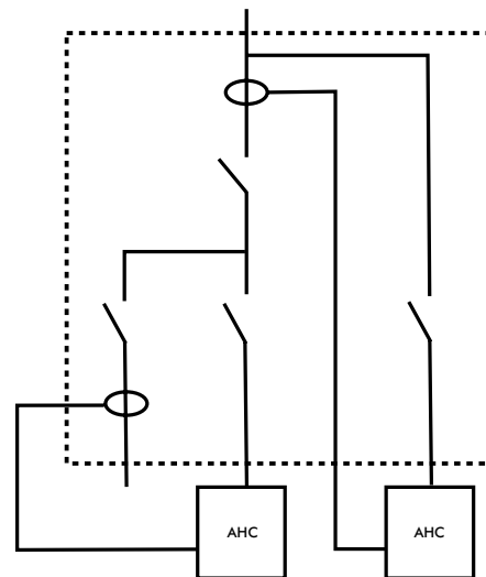
Figure 7 - Cascade configuration
