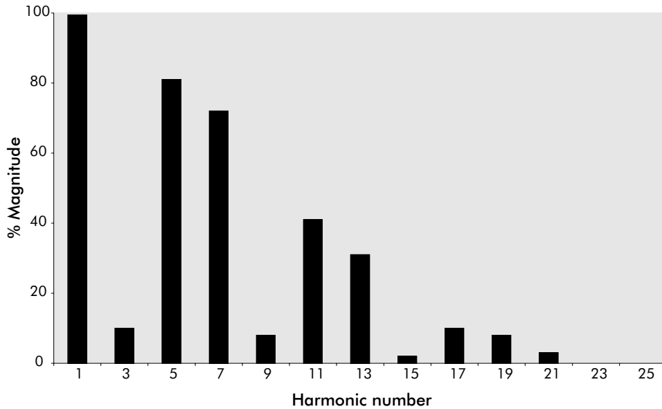
Figure 11 - Typical uncorrected variable speed drive load
