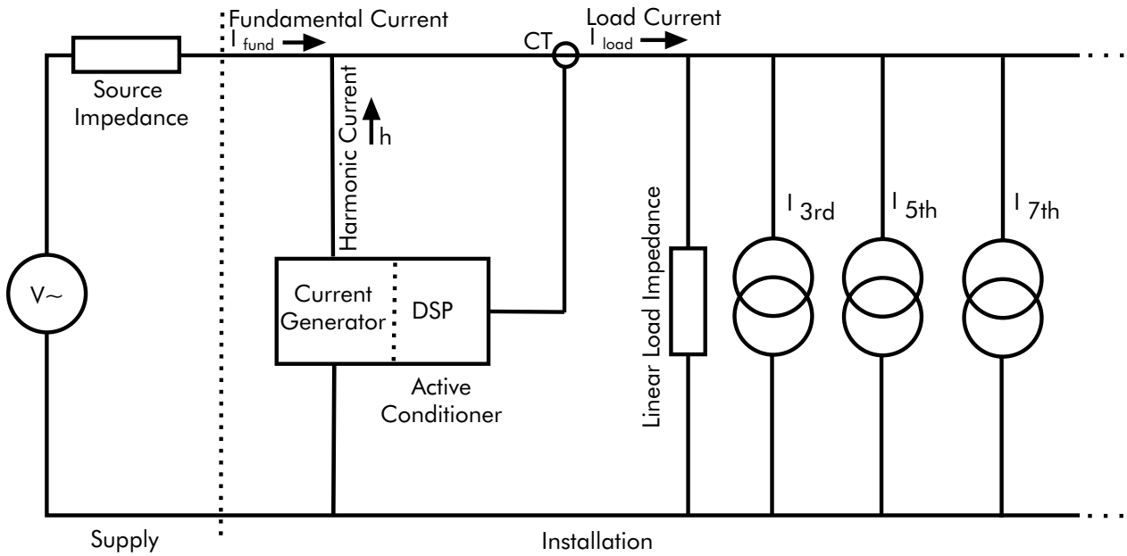
Figure 1 - Parallel active harmonic conditioner
