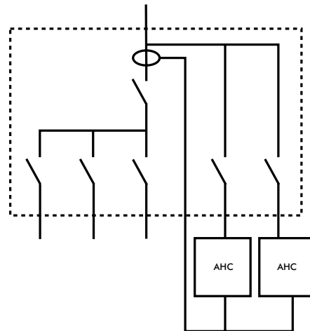
Figure 6 - Parallel configuration
