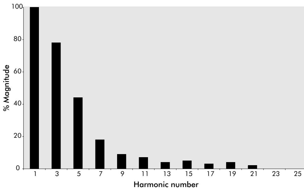
Figure 8 - Uncorrected profile of PC type loads
