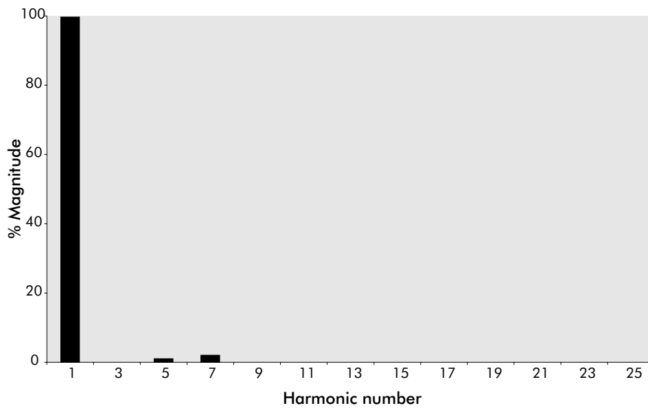
Figure 9 - Completely corrected PC type load
